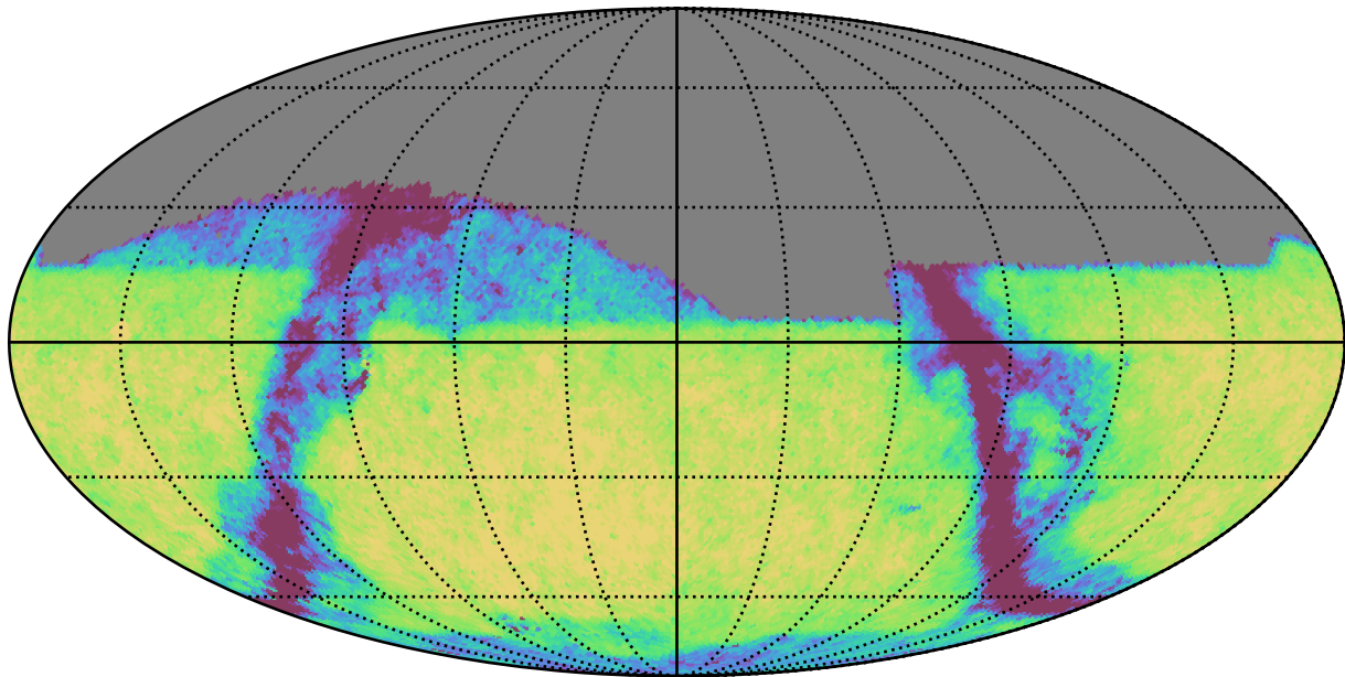
telescope_jerk_v3.5_10yrs Yr 1 z band: Exgal_CoaddM5
