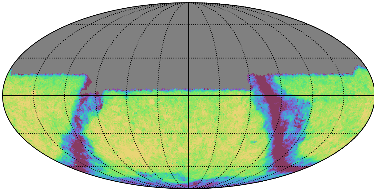
telescope_jerk_v3.5_10yrs Yr 1 y band: Exgal_CoaddM5
