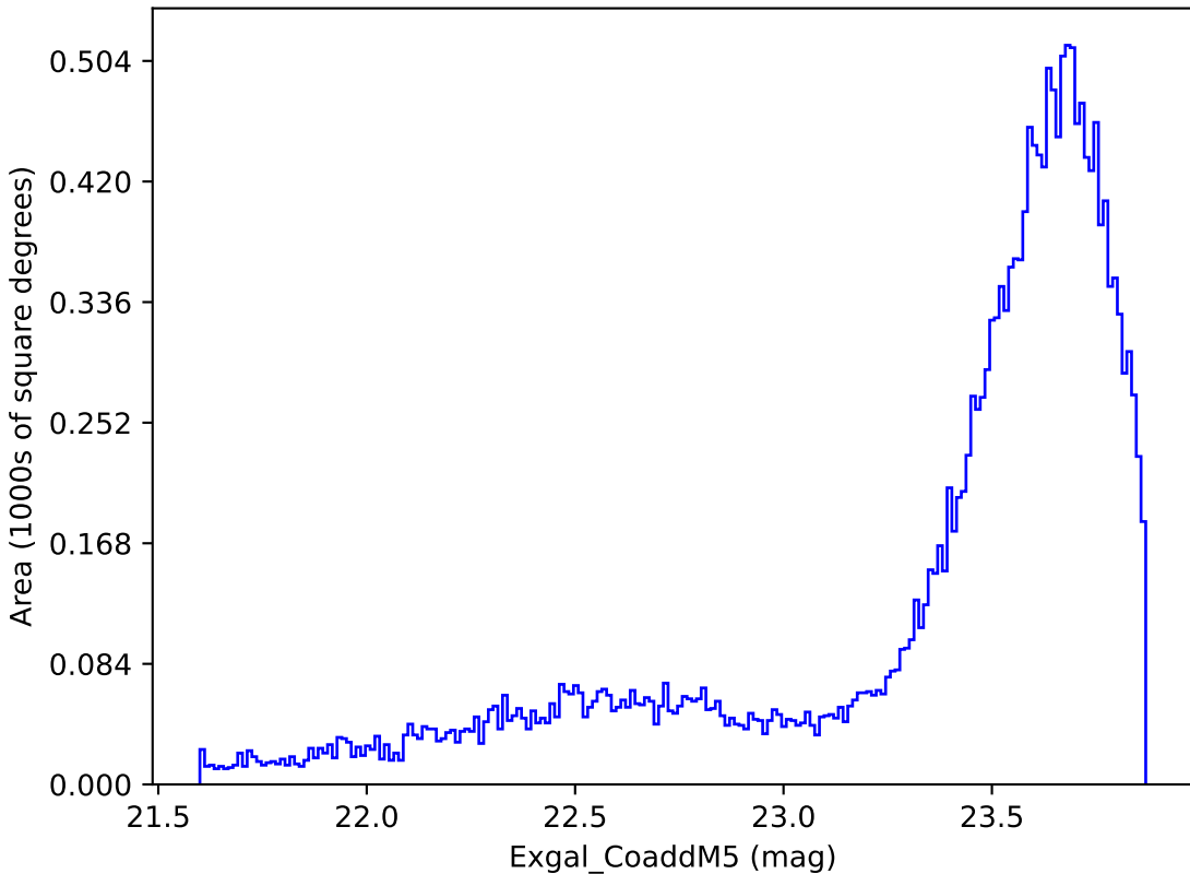
telescope_jerk_v3.5_10yrs Yr 1 y band: Exgal_CoaddM5
