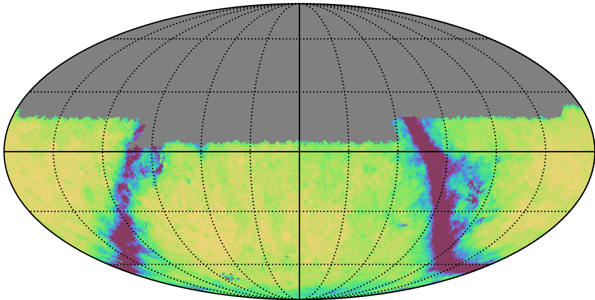
telescope_jerk_v3.5_10yrs Yr 1 u band: Exgal_CoaddM5
