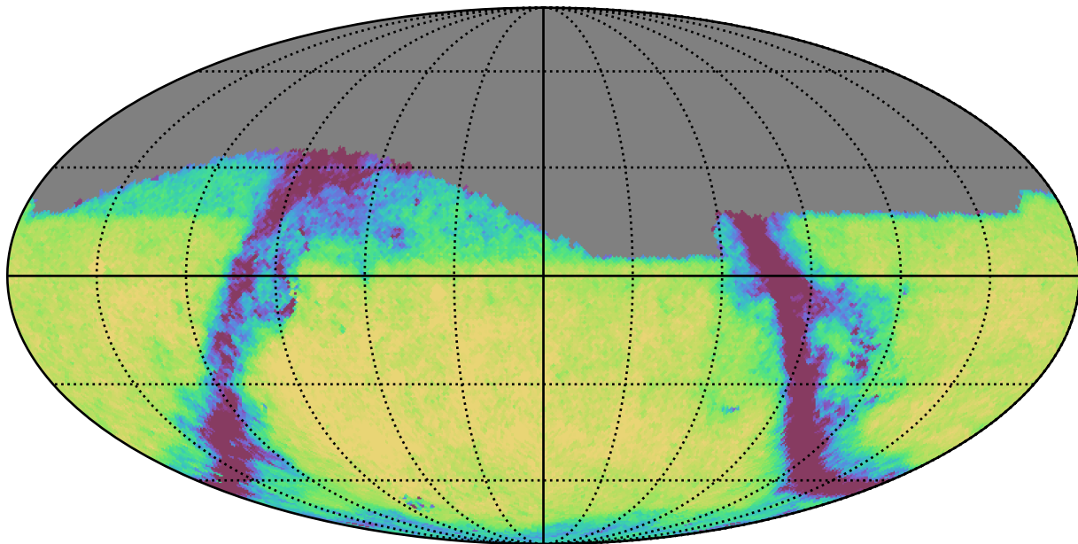
telescope_jerk_v3.5_10yrs Yr 1 r band: Exgal_CoaddM5
