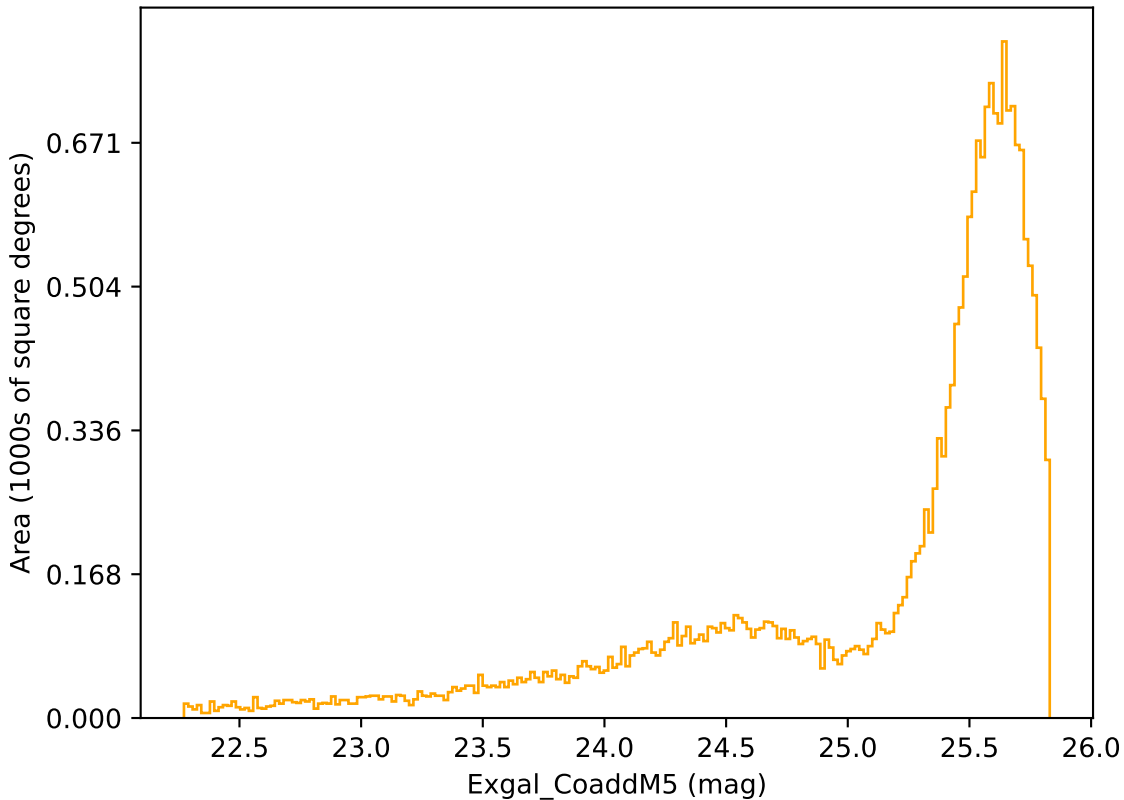
telescope_jerk_v3.5_10yrs Yr 1 r band: Exgal_CoaddM5
