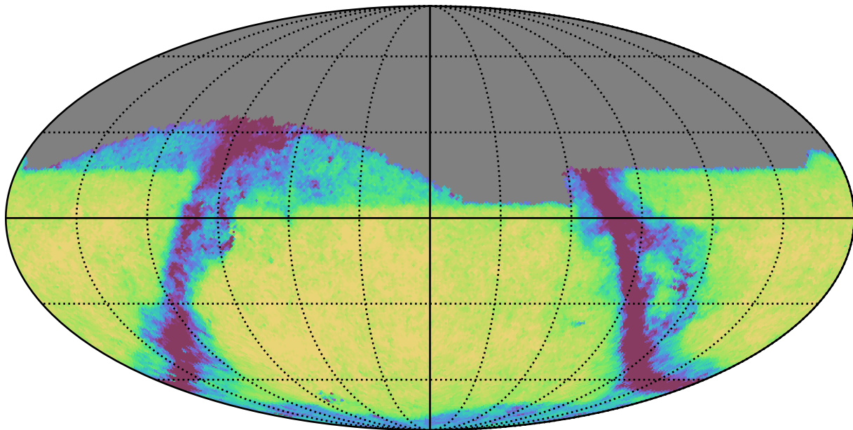
telescope_jerk_v3.5_10yrs Yr 1 i band: Exgal_CoaddM5
