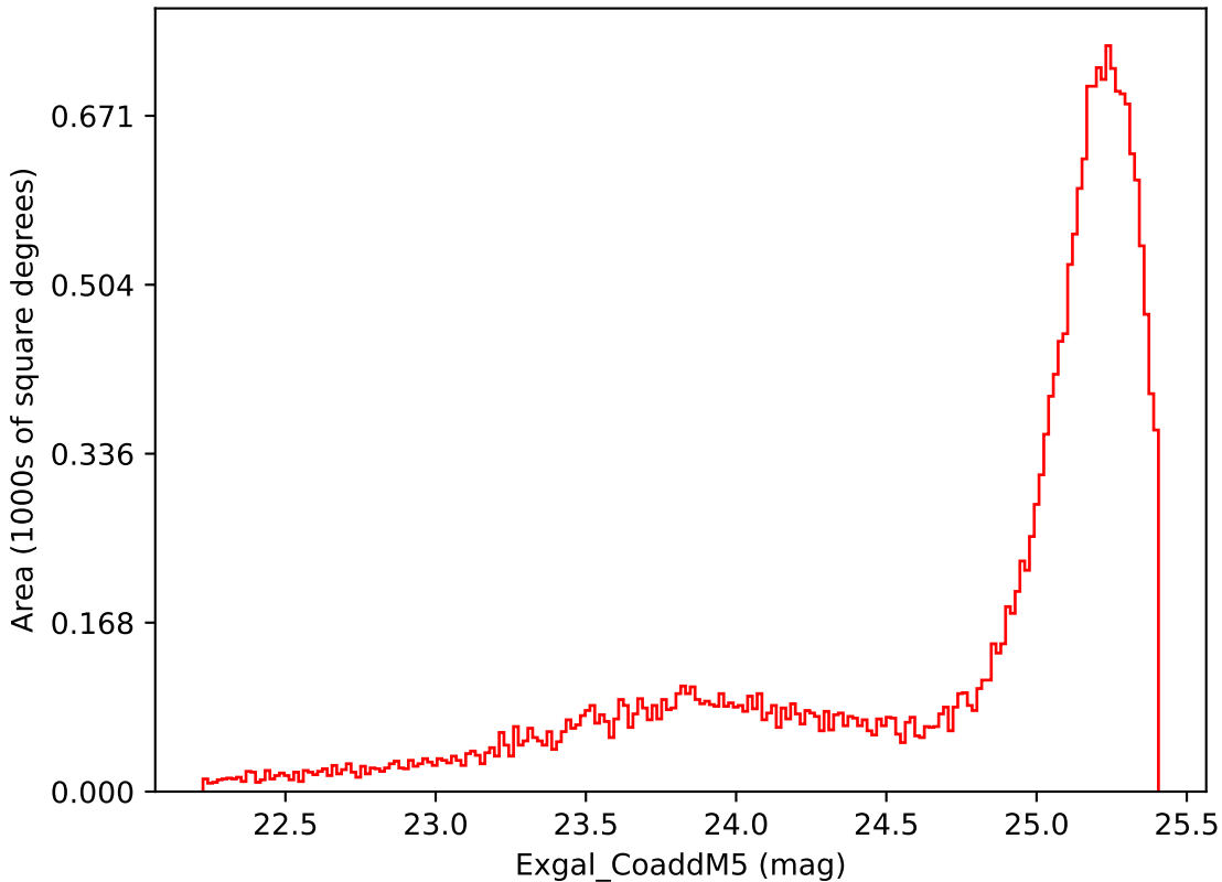
telescope_jerk_v3.5_10yrs Yr 1 i band: Exgal_CoaddM5
