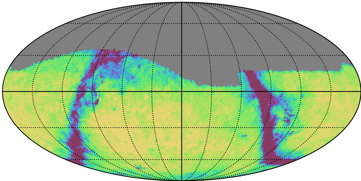
telescope_jerk_v3.5_10yrs Yr 1 g band: Exgal_CoaddM5
