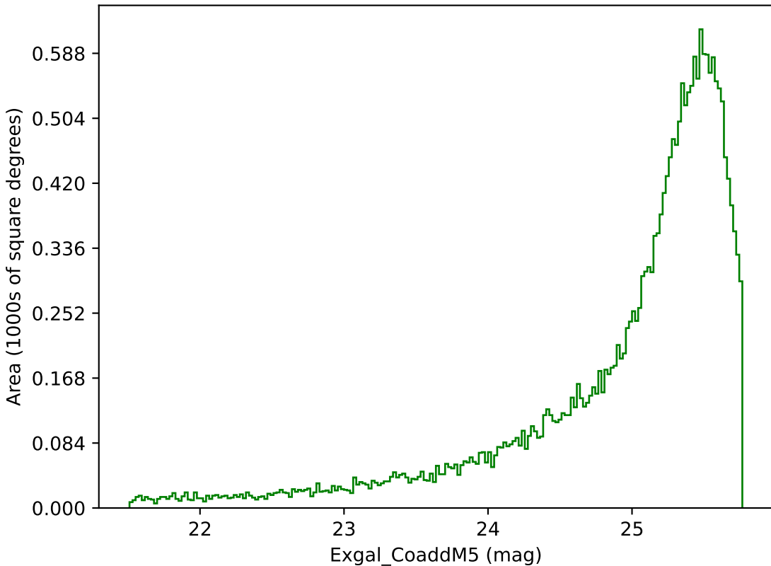
telescope_jerk_v3.5_10yrs Yr 1 g band: Exgal_CoaddM5
