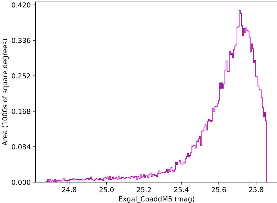
telescope_jerk_v3.5_10yrs WFD z band: Exgal_CoaddM5
