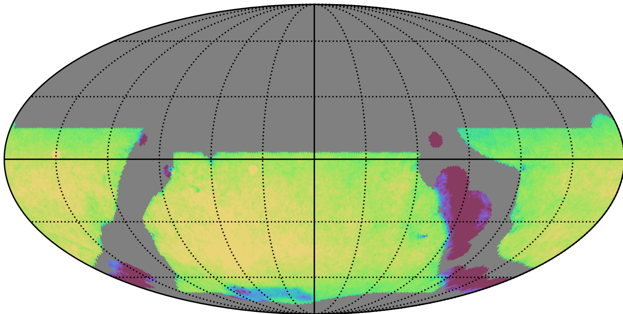
telescope_jerk_v3.5_10yrs WFD y band: Exgal_CoaddM5
