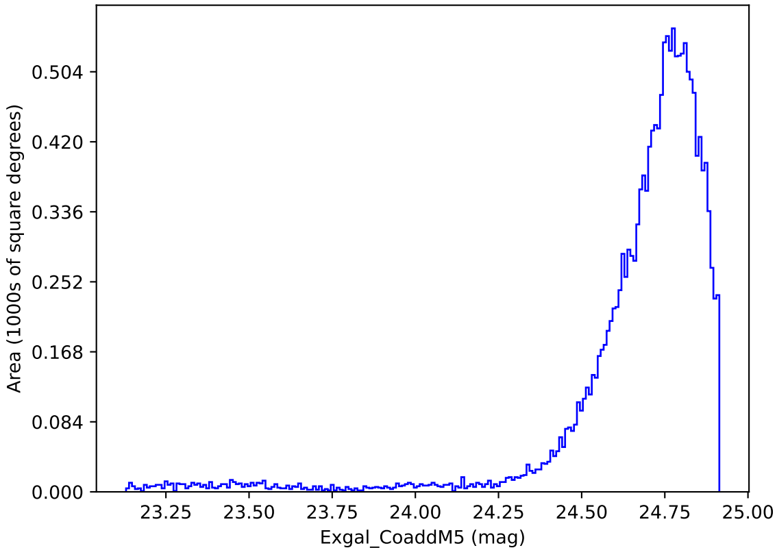
telescope_jerk_v3.5_10yrs WFD y band: Exgal_CoaddM5
