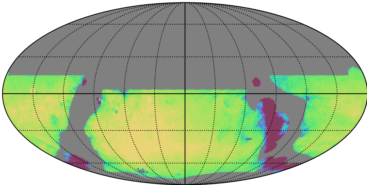
telescope_jerk_v3.5_10yrs WFD r band: Exgal_CoaddM5
