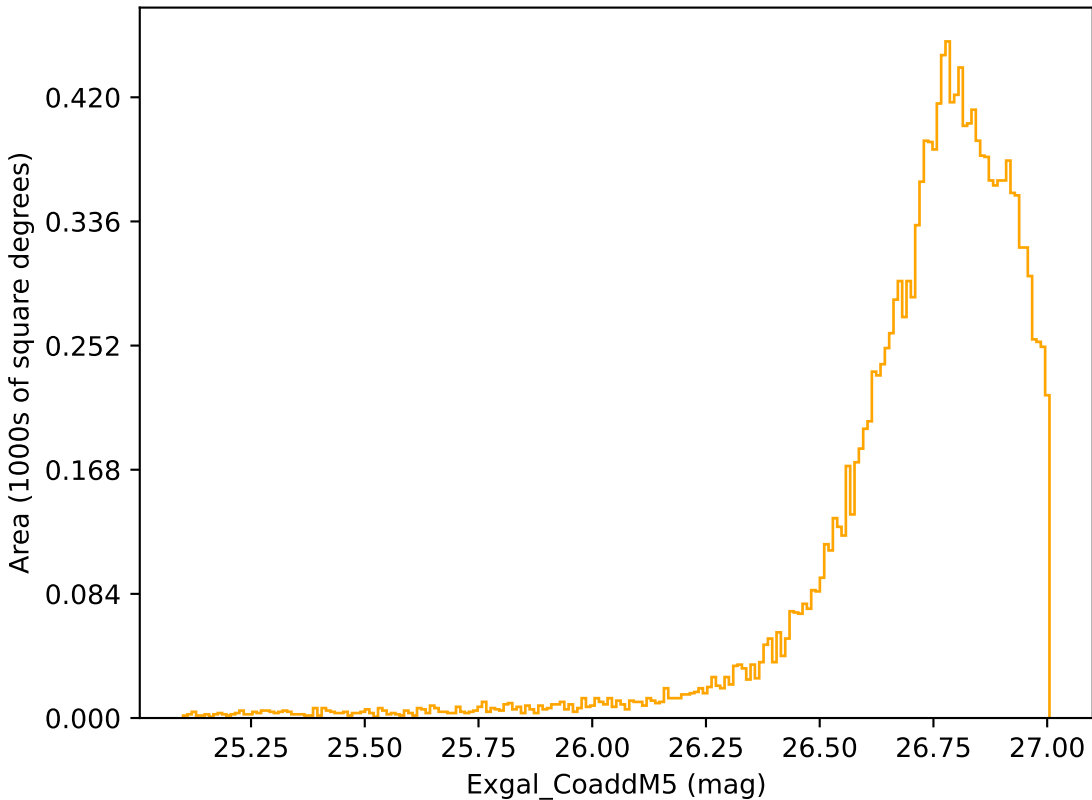
telescope_jerk_v3.5_10yrs WFD r band: Exgal_CoaddM5
