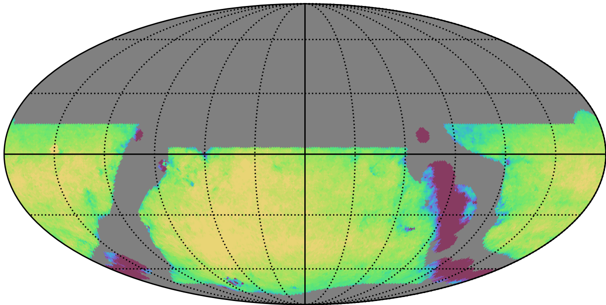
telescope_jerk_v3.5_10yrs WFD i band: Exgal_CoaddM5
