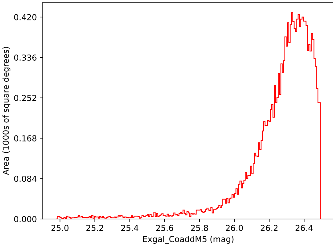
telescope_jerk_v3.5_10yrs WFD i band: Exgal_CoaddM5
