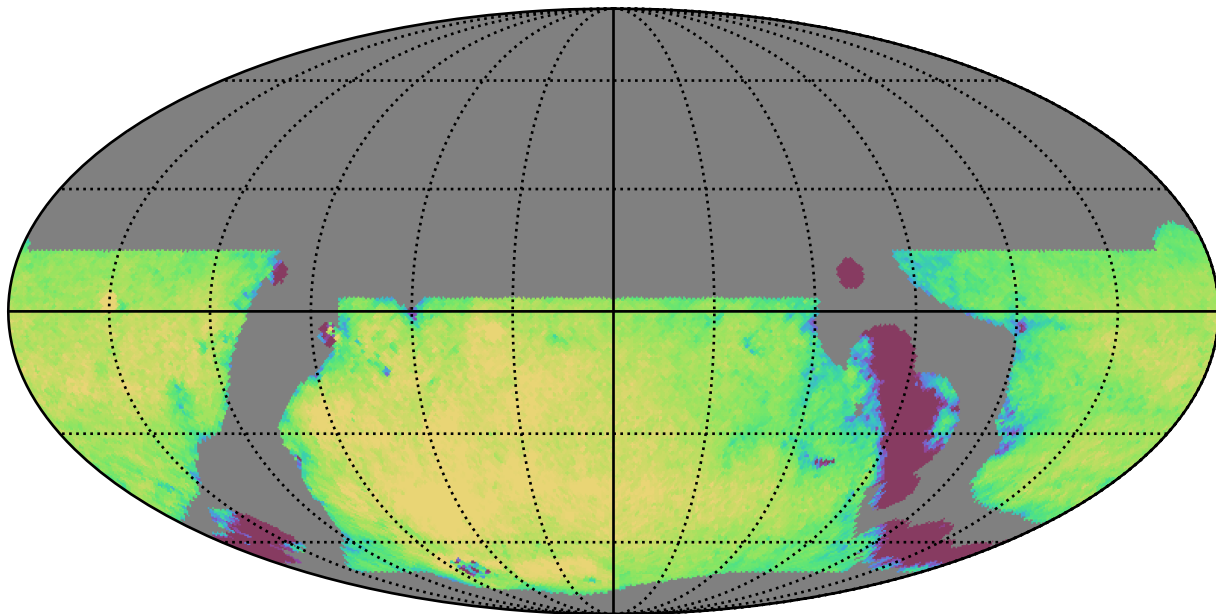
telescope_jerk_v3.5_10yrs WFD g band: Exgal_CoaddM5
