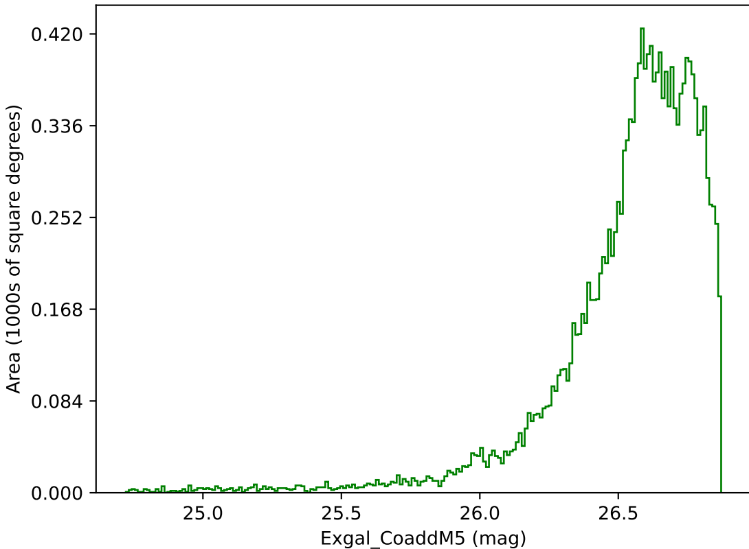
telescope_jerk_v3.5_10yrs WFD g band: Exgal_CoaddM5
