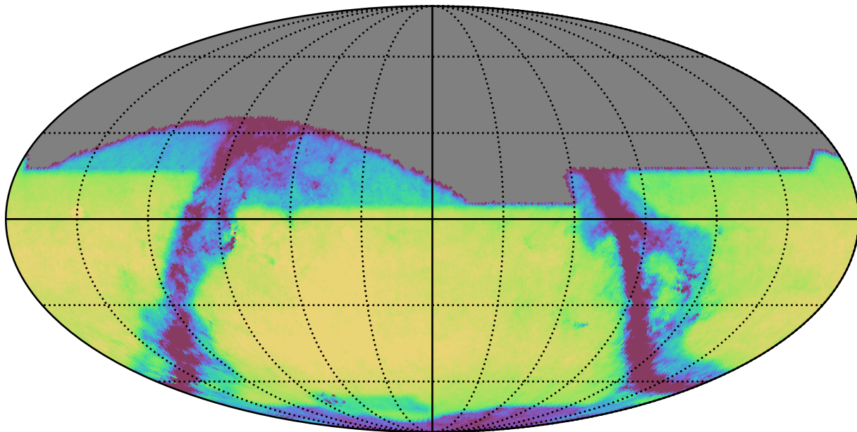
telescope_jerk_v3.5_10yrs All sky z band: Exgal_CoaddM5
