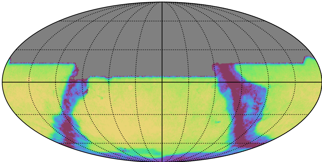
telescope_jerk_v3.5_10yrs All sky y band: Exgal_CoaddM5
