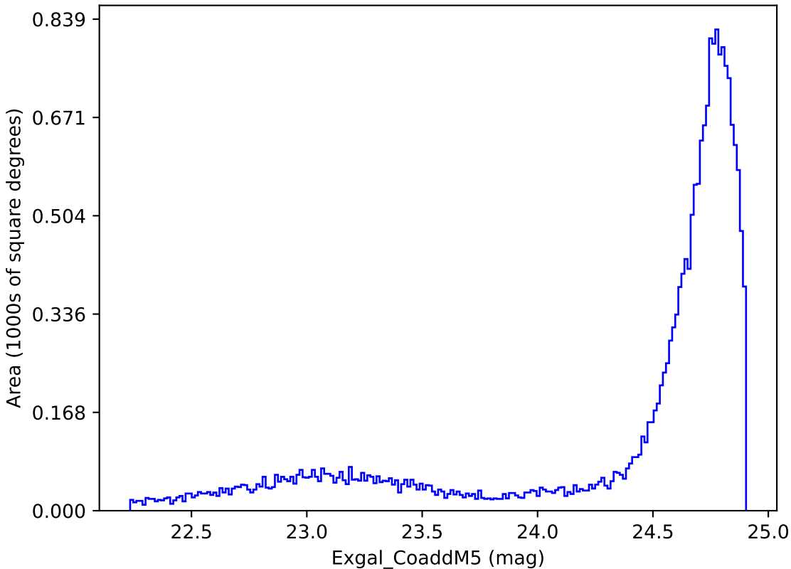
telescope_jerk_v3.5_10yrs All sky y band: Exgal_CoaddM5
