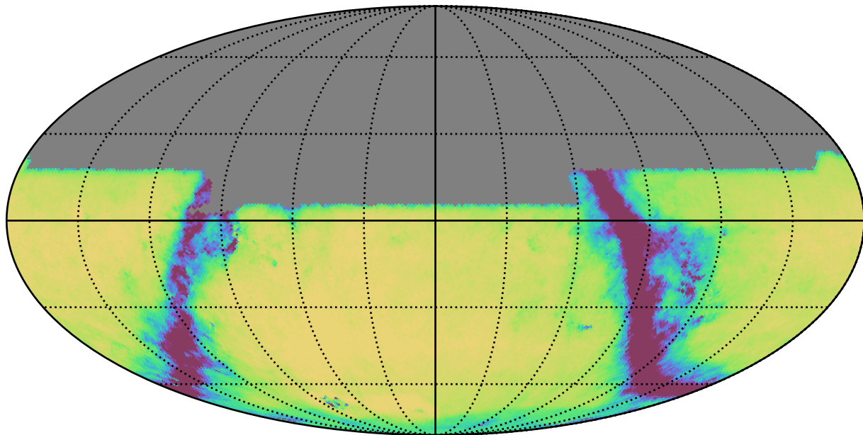
telescope_jerk_v3.5_10yrs All sky u band: Exgal_CoaddM5
