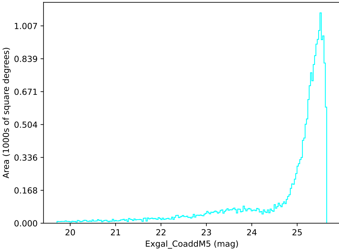
telescope_jerk_v3.5_10yrs All sky u band: Exgal_CoaddM5
