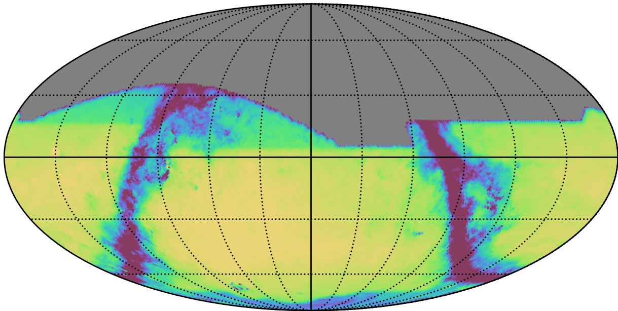
telescope_jerk_v3.5_10yrs All sky r band: Exgal_CoaddM5
