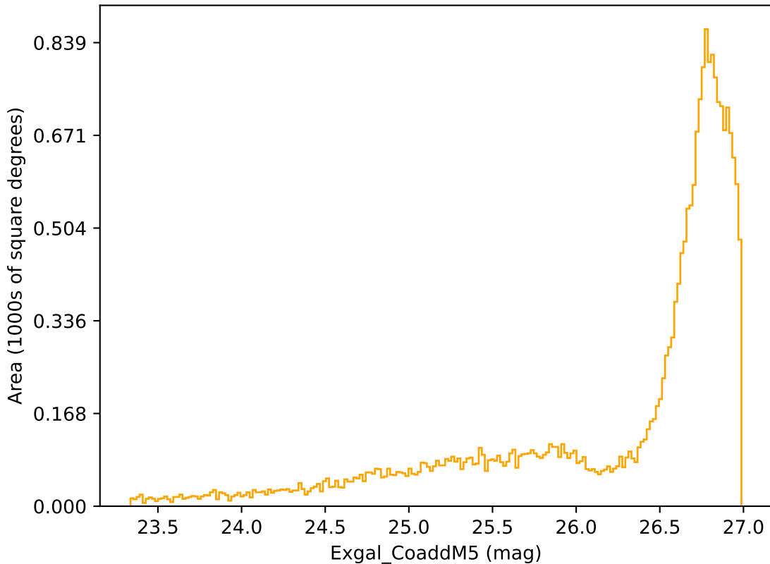
telescope_jerk_v3.5_10yrs All sky r band: Exgal_CoaddM5
