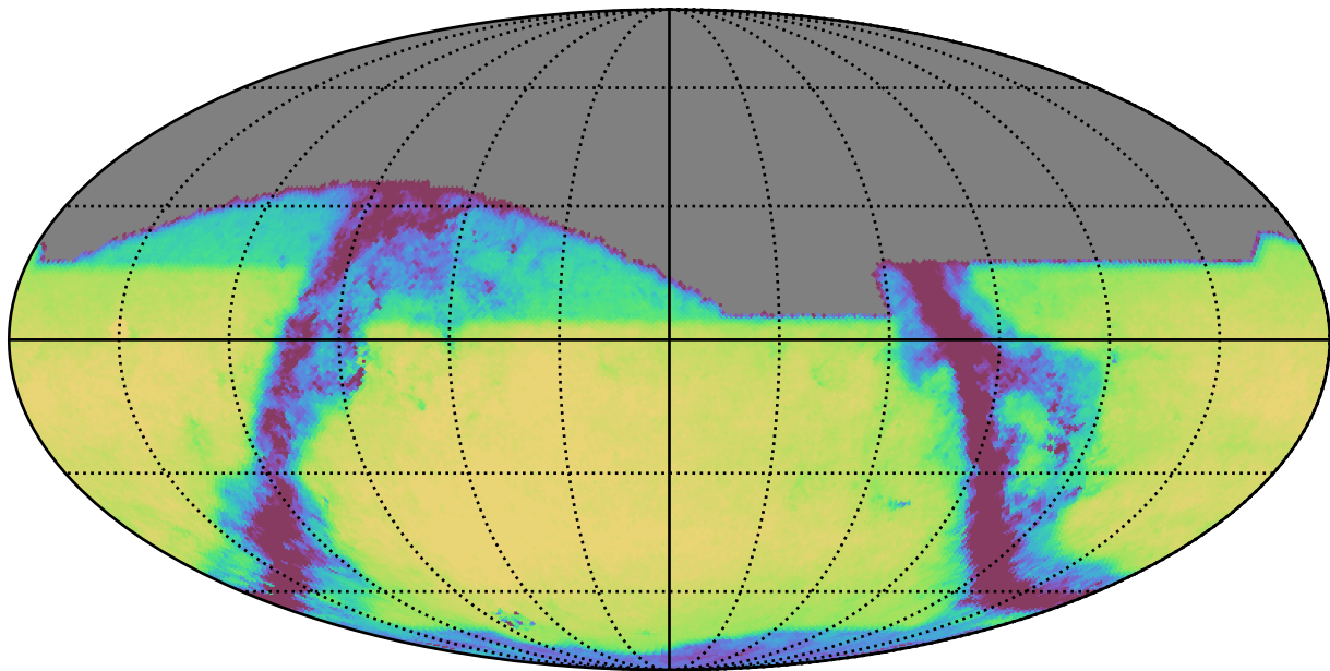
telescope_jerk_v3.5_10yrs All sky i band: Exgal_CoaddM5
