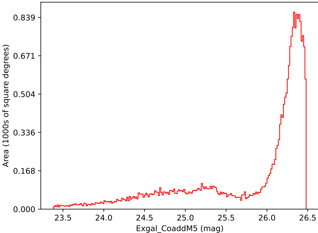
telescope_jerk_v3.5_10yrs All sky i band: Exgal_CoaddM5
