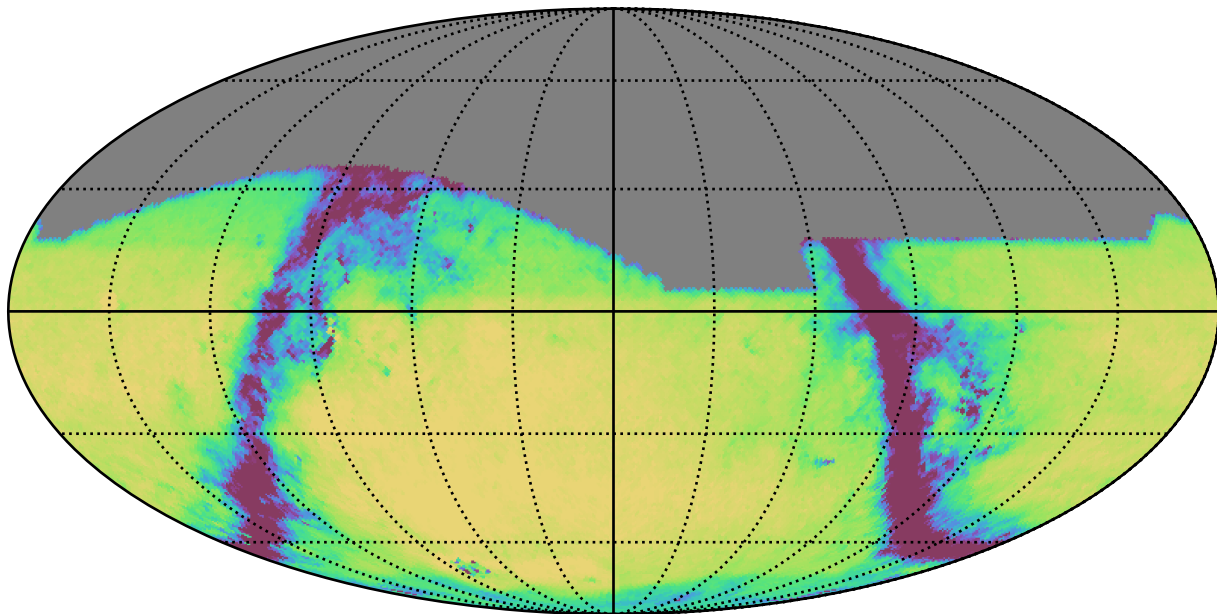
telescope_jerk_v3.5_10yrs All sky g band: Exgal_CoaddM5
