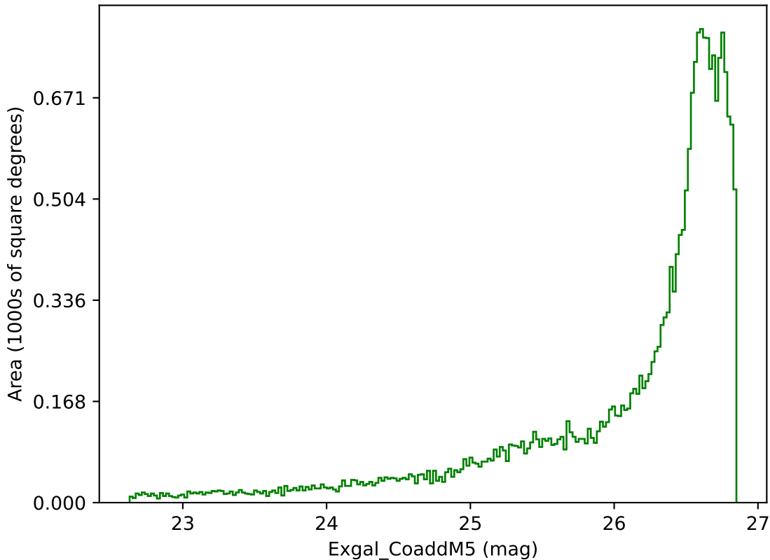
telescope_jerk_v3.5_10yrs All sky g band: Exgal_CoaddM5
