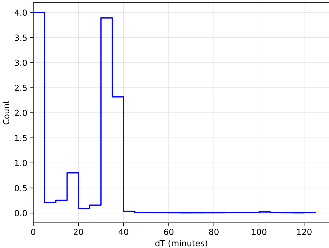
1e6 telescope_jerk_v3.5_10yrs WFD: DeltaT Histogram
