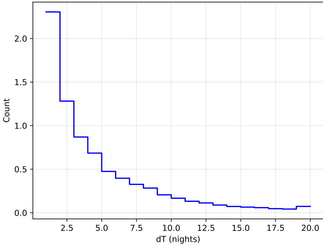
telescope_jerk_v3.5_10yrs WFD all bands: DeltaNight Histogram 1e6
