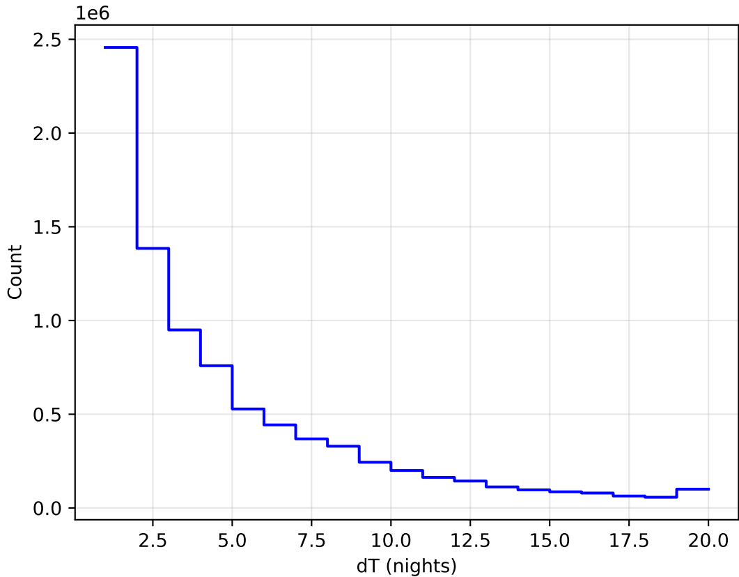
telescope_jerk_v3.5_10yrs All sky all bands: DeltaNight Histogram
