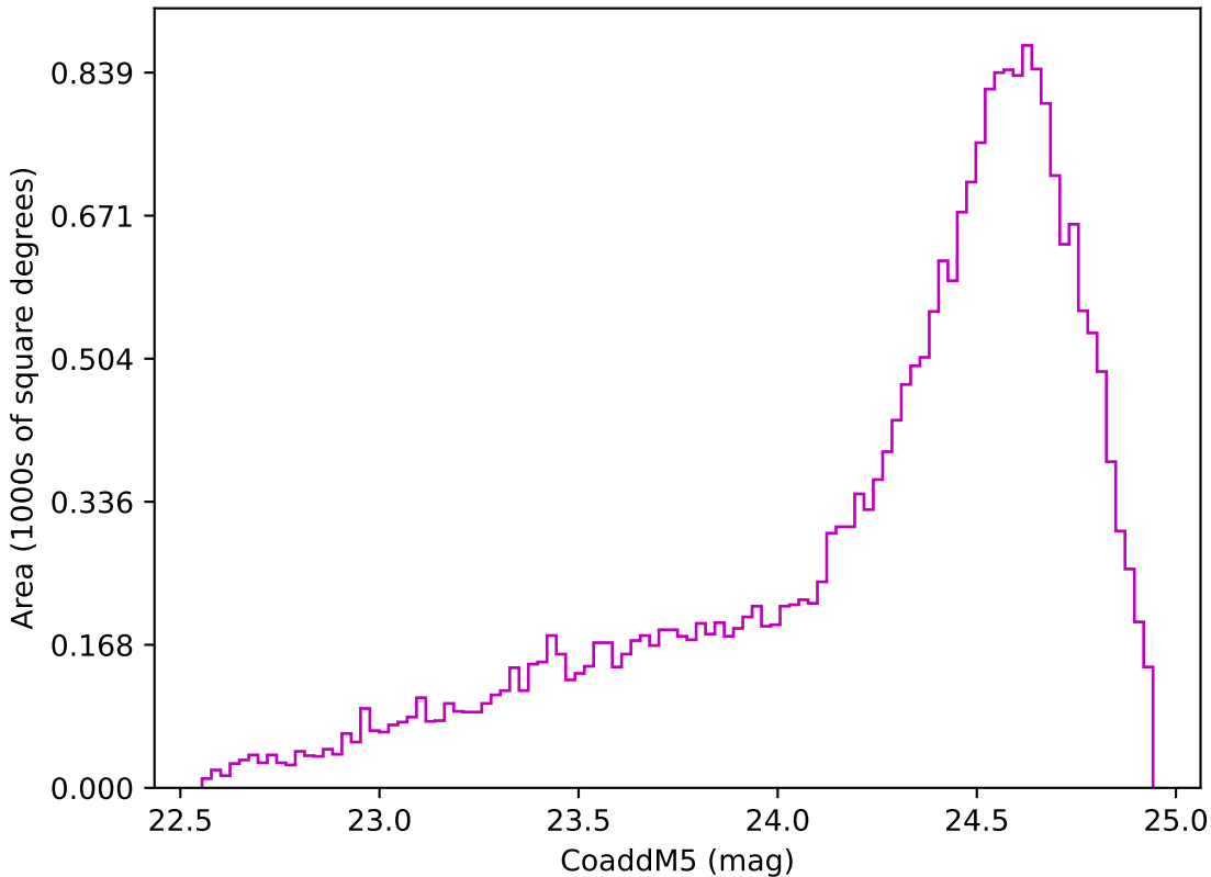
telescope_jerk_v3.5_10yrs Yr 3-4 z band: CoaddM5
