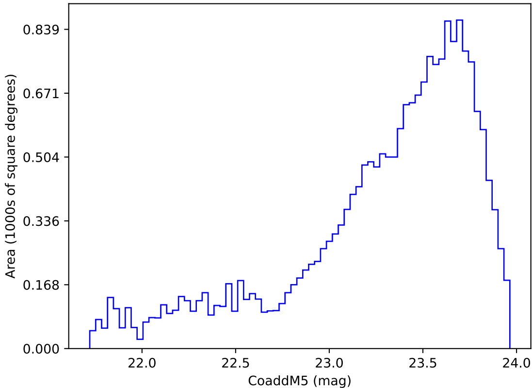
telescope_jerk_v3.5_10yrs Yr 3-4 y band: CoaddM5
