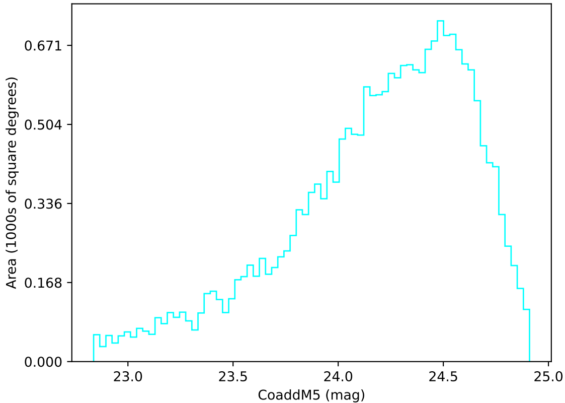
telescope_jerk_v3.5_10yrs Yr 3-4 u band: CoaddM5
