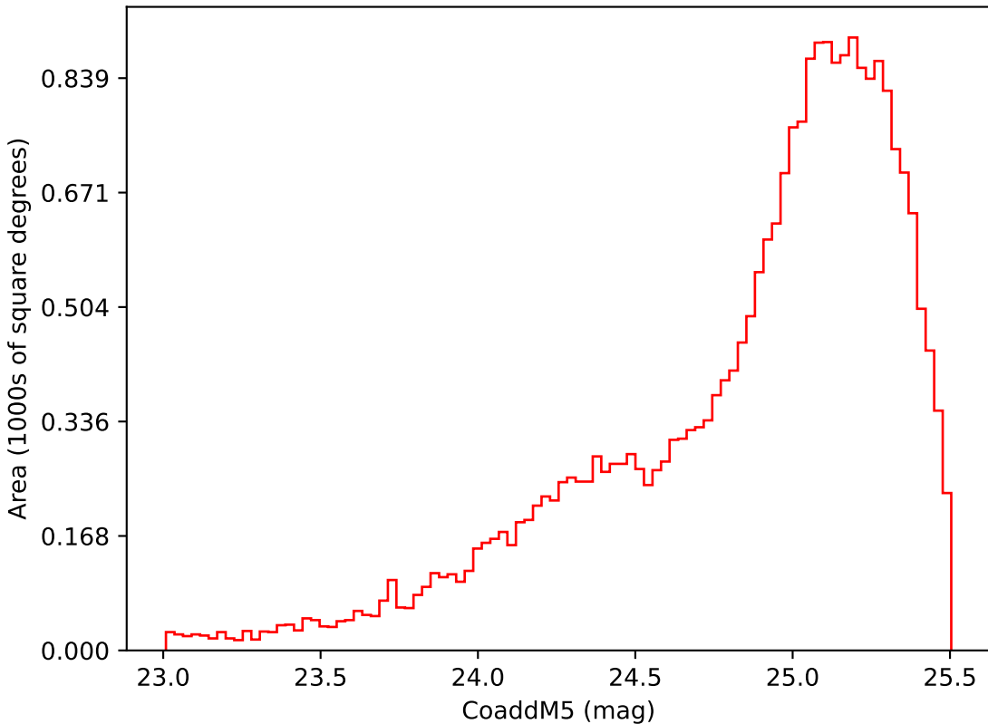
telescope_jerk_v3.5_10yrs Yr 3-4 i band: CoaddM5
