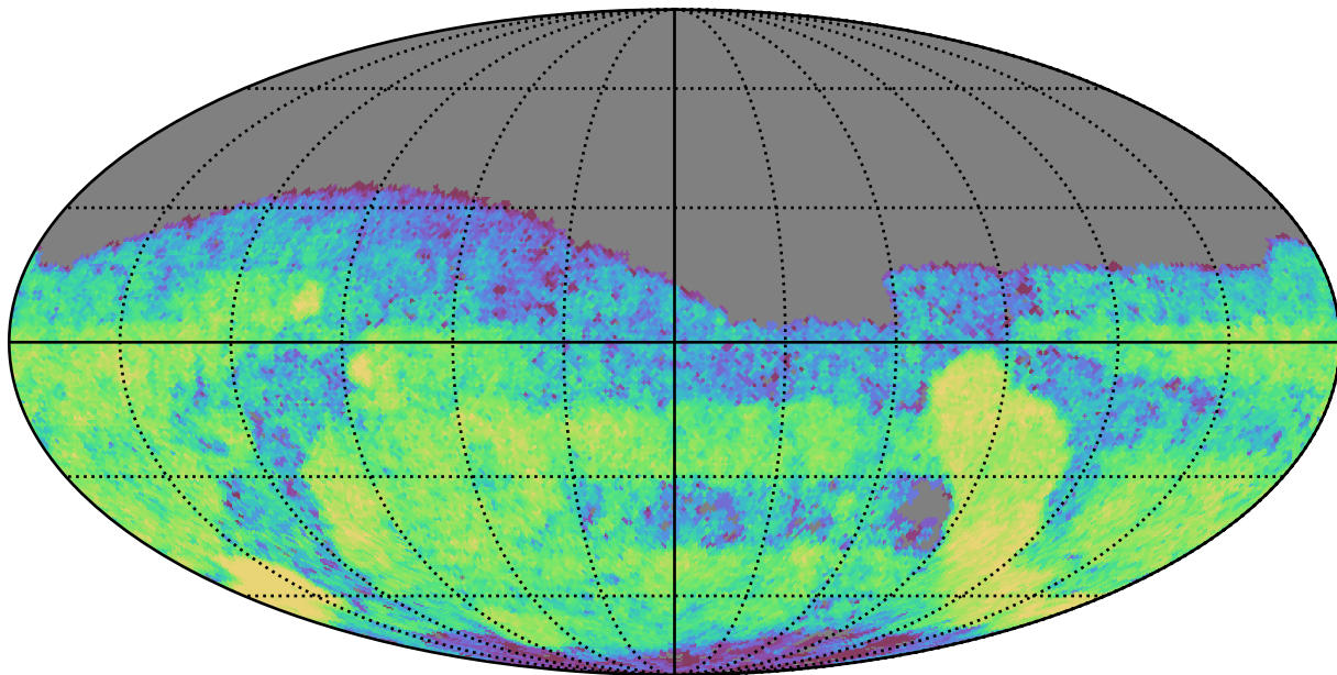
telescope_jerk_v3.5_10yrs Yr 3-4 g band: CoaddM5
