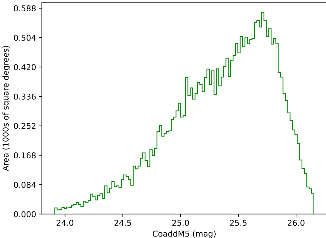
telescope_jerk_v3.5_10yrs Yr 3-4 g band: CoaddM5
