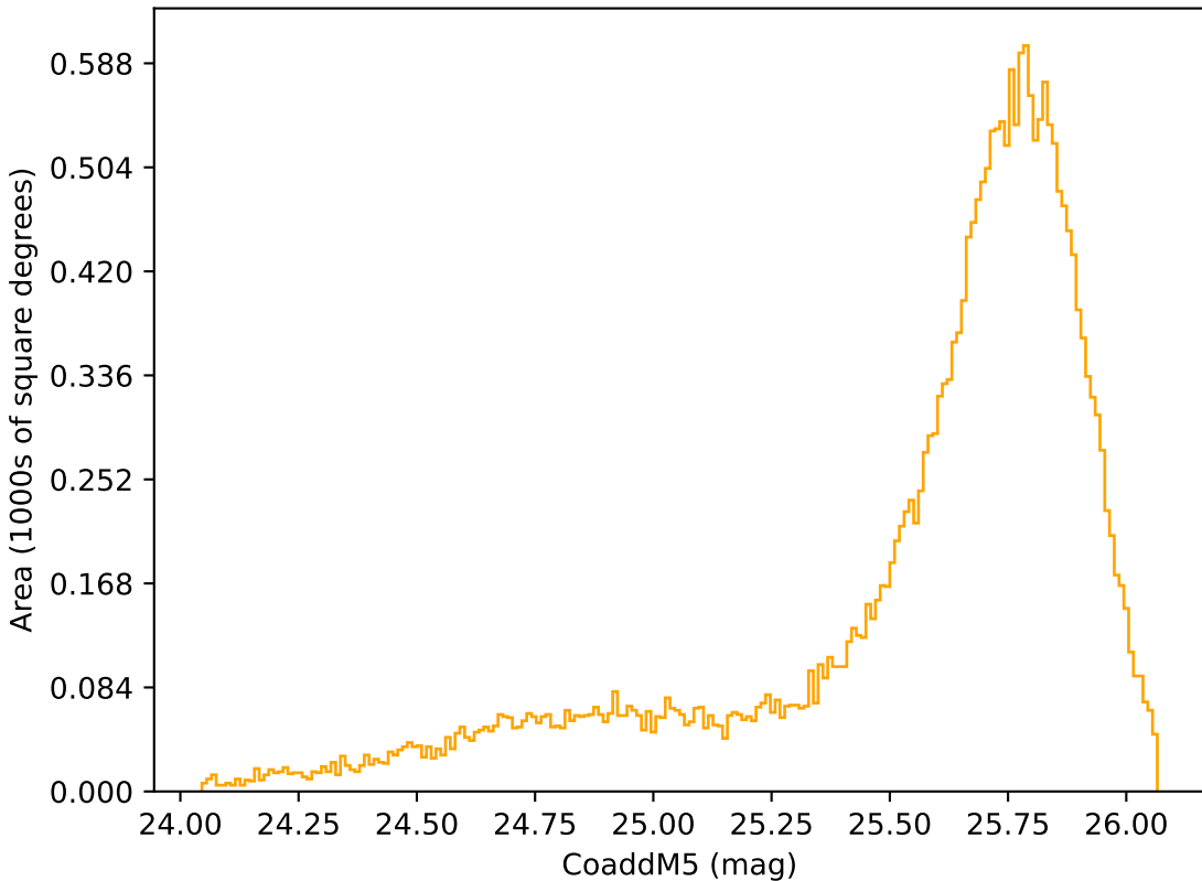
telescope_jerk_v3.5_10yrs Yr 1 r band: CoaddM5
