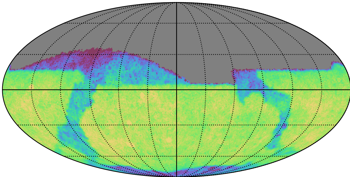
telescope_jerk_v3.5_10yrs Yr 1 i band: CoaddM5
