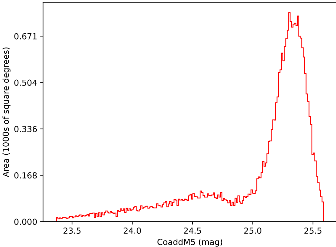
telescope_jerk_v3.5_10yrs Yr 1 i band: CoaddM5
