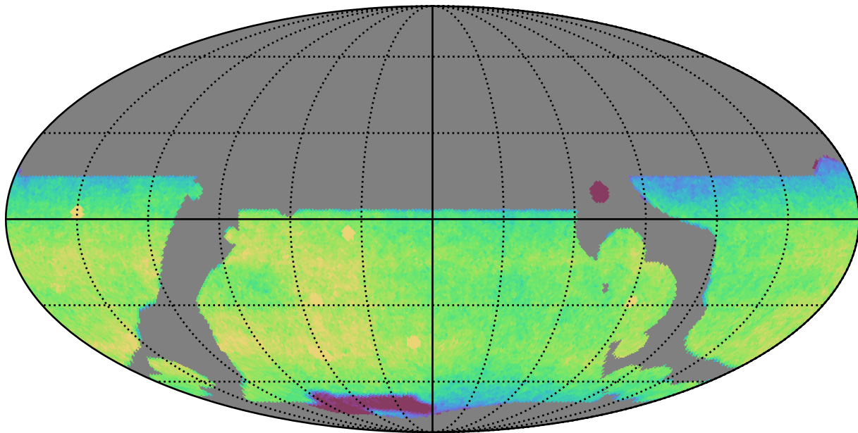
telescope_jerk_v3.5_10yrs WFD z band: CoaddM5
