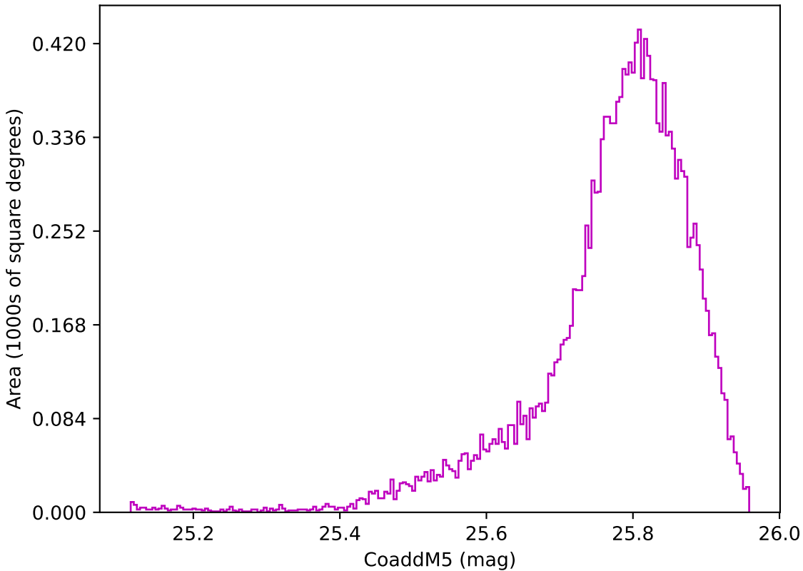
telescope_jerk_v3.5_10yrs WFD z band: CoaddM5
