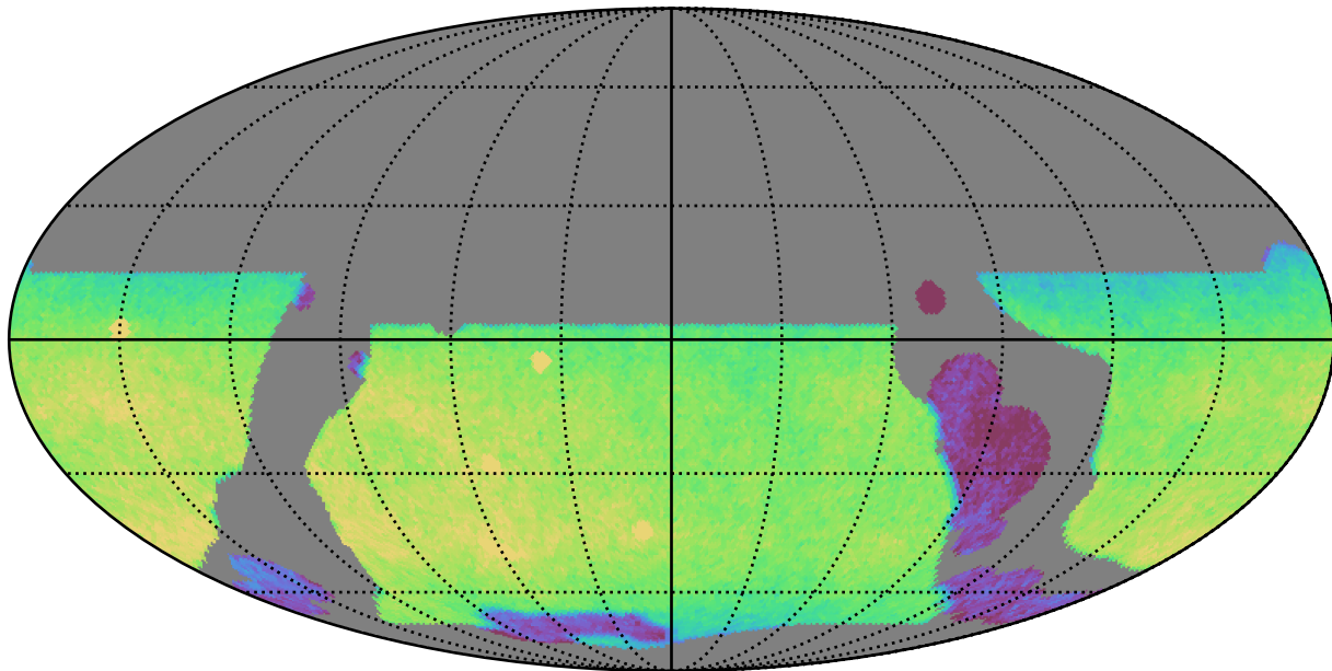
telescope_jerk_v3.5_10yrs WFD y band: CoaddM5
