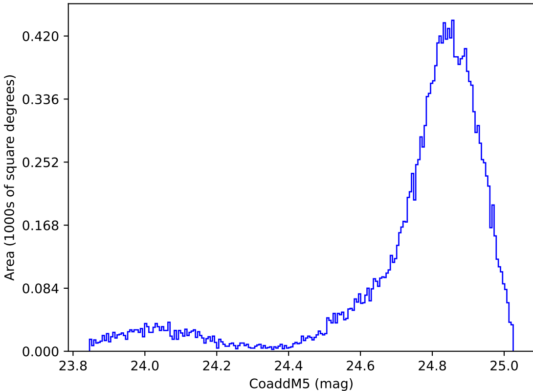
telescope_jerk_v3.5_10yrs WFD y band: CoaddM5
