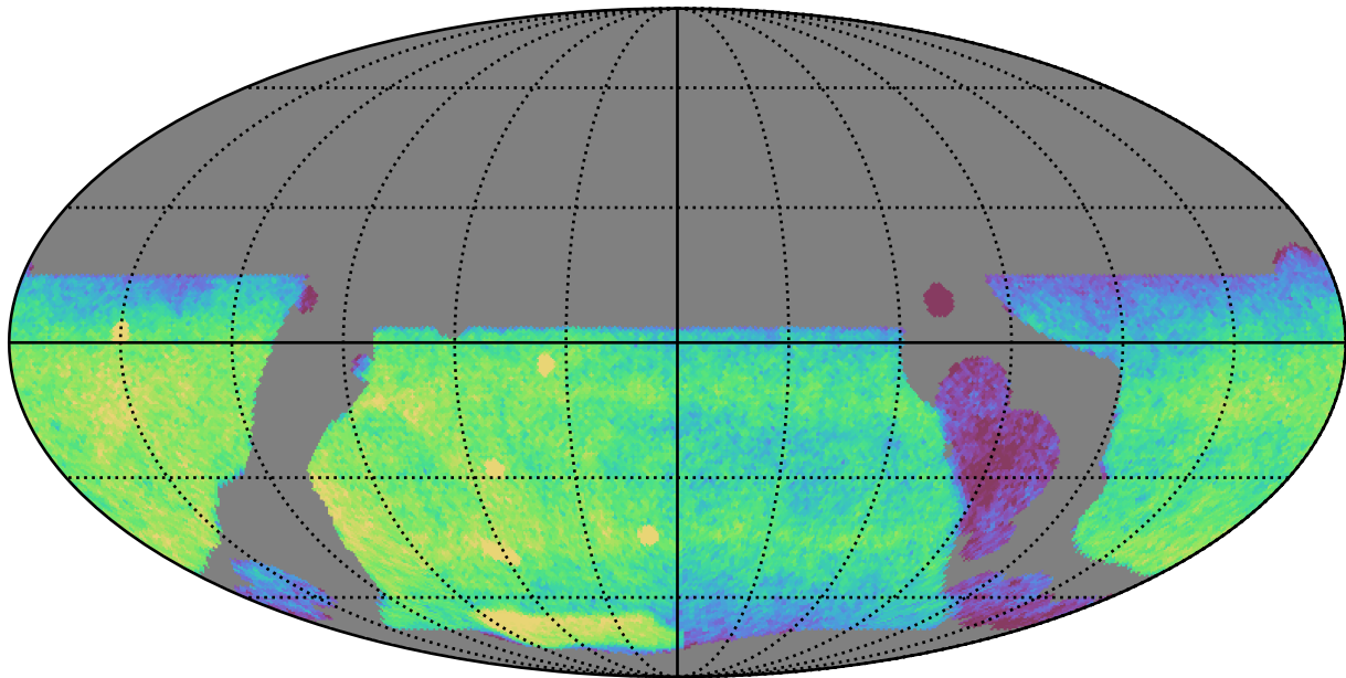
telescope_jerk_v3.5_10yrs WFD u band: CoaddM5
