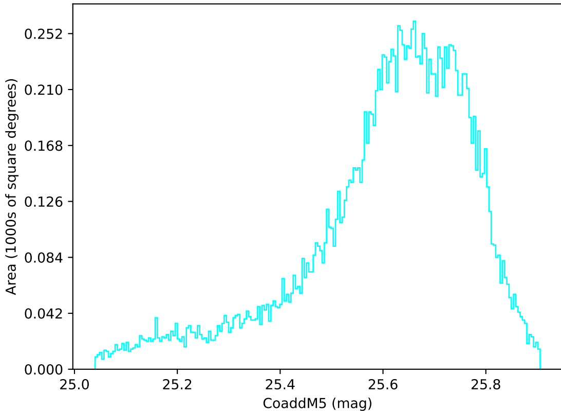
telescope_jerk_v3.5_10yrs WFD u band: CoaddM5
