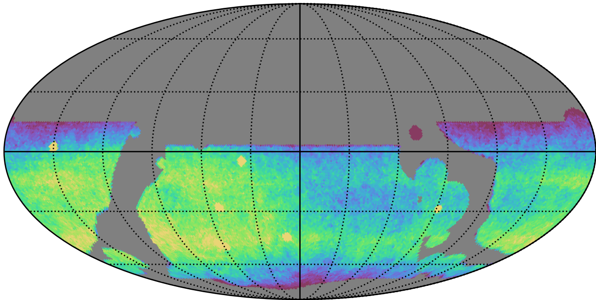
telescope_jerk_v3.5_10yrs WFD r band: CoaddM5
