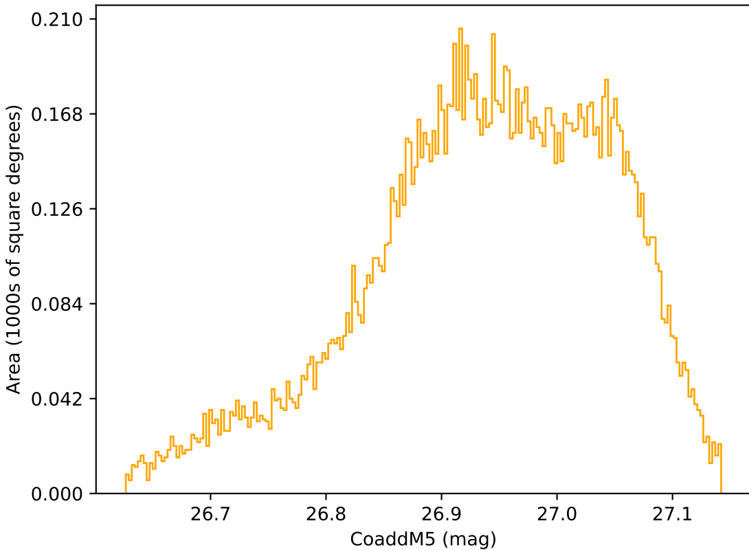
telescope_jerk_v3.5_10yrs WFD r band: CoaddM5
